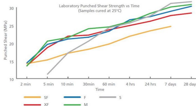
Figure 3 - Punched Shear Strength v's Time
