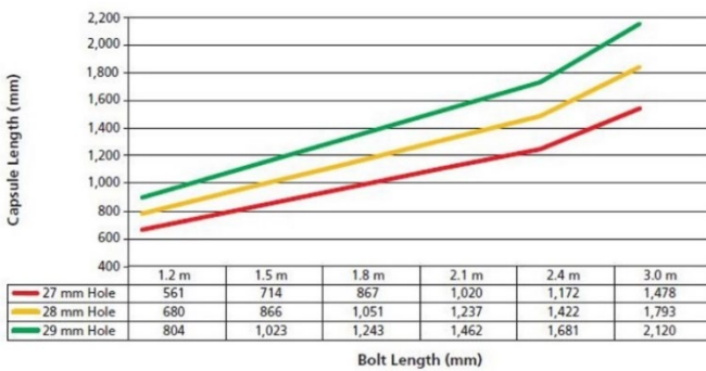
Figure 4 - Encapsulation Volume
